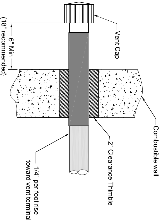
HORIZONTAL THROUGH SIDEWALL (Combustible Wall)
